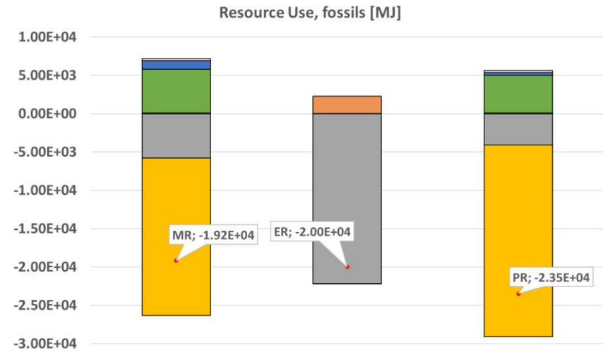
Figure 7. Management of 1 tonne of sorted large-format PE film waste through mechanical recycling (MR; LDPE regranulate production), energy recovery (ER; incineration), and physical recycling (PR; solvent-based separation/dissolution and subsequent production of LDPE granulate): Climate Change, Particulate Matter, Acidification, and Resource Use, fossils impact indicators. Negative values represent savings, while positive ones represent burdens. See Table 1 for a description of the different treatment scenarios and technologies.
